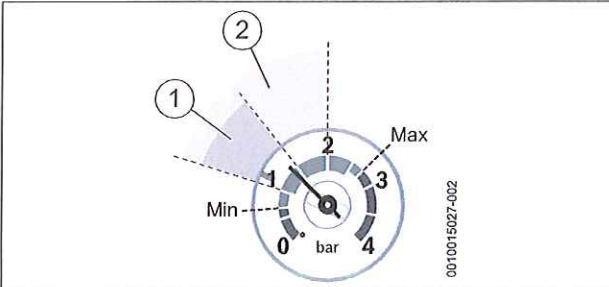
Fig. 2 Pressure gauge for checking the operating pressure
