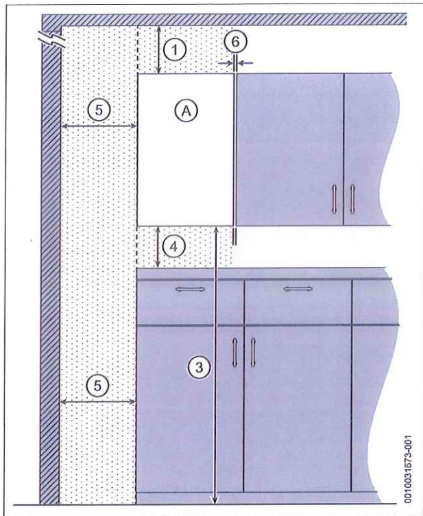
Fig. 11 Reduced front maintenance clearances - Front view
