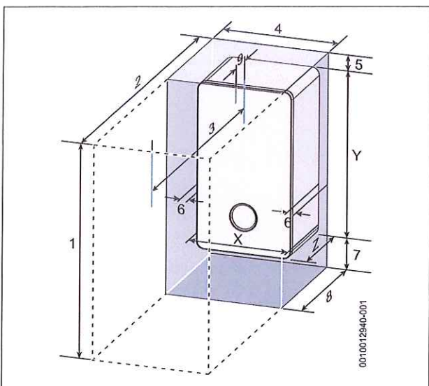
Fig. 9 Appliance minimum clearances
