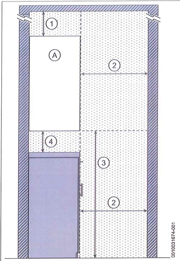
Fig. 10 Reduced front maintenance clearances - Side view
