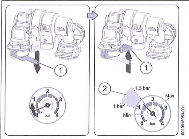
Fig. 5 Keyless filling link
