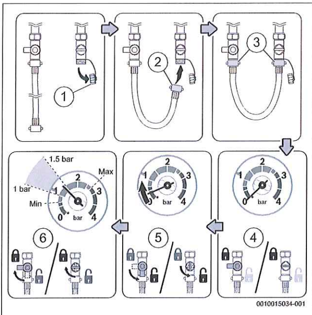
Fig. 4 External filling loop
